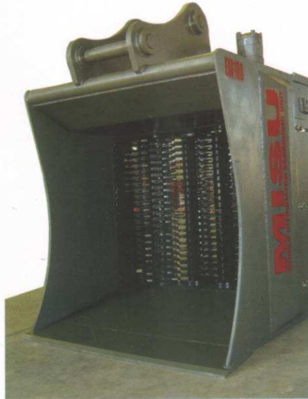
MISU's screening unit uses components made from abrasive resistant Hardox 500 to ensure longevity.
